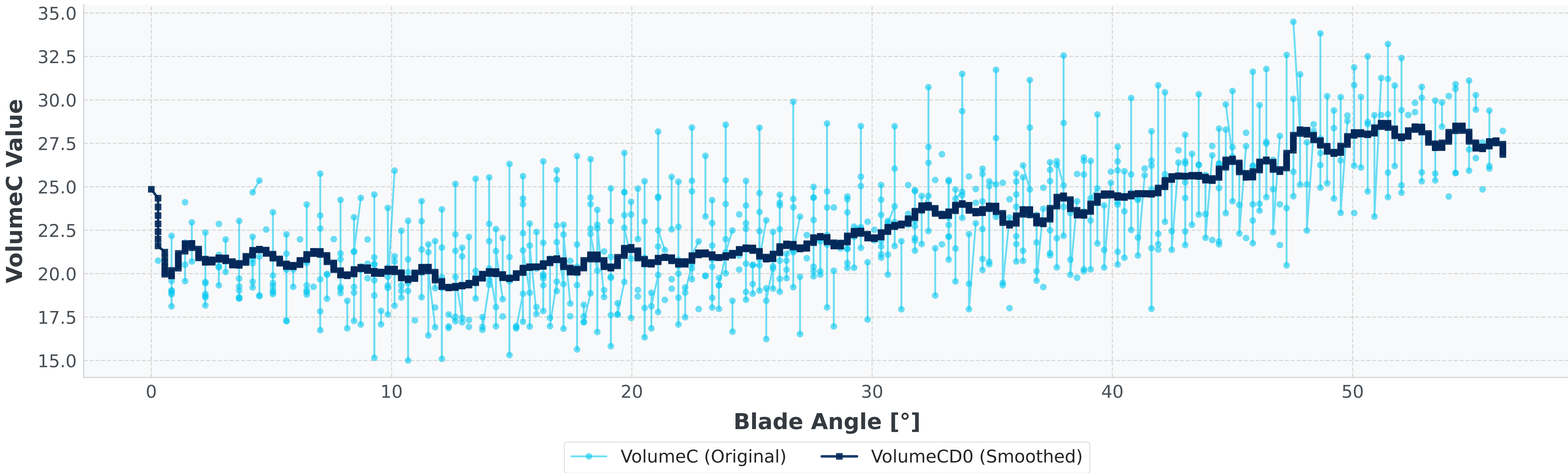
Cavity - VolumeC (BLD Phase Averaged)
