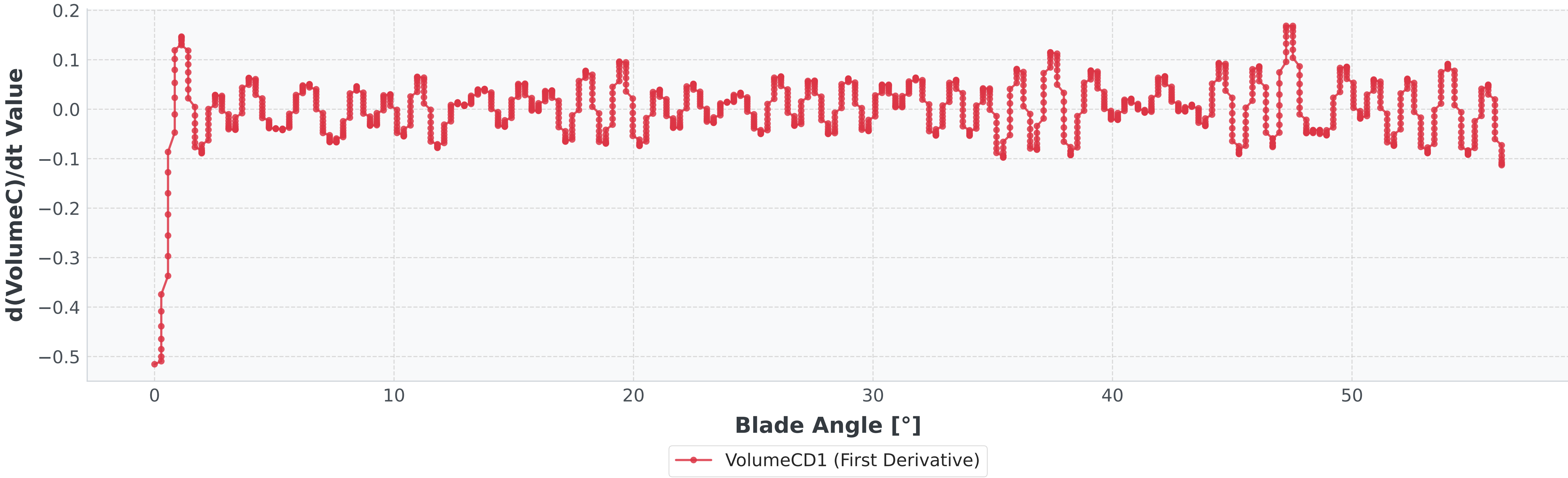
Cavity - VolumeC First Derivative (BLD)
